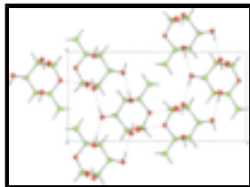
Fig. 3. Packing diagram of the title compound projected along the a -axis.
